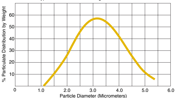
Typical Contaminant Challenge to a Particulate Filter
